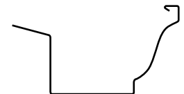
GUTTER WITH BACK FLANGE 1" or 1-1/2" (25.4mm or 38.1mm)
